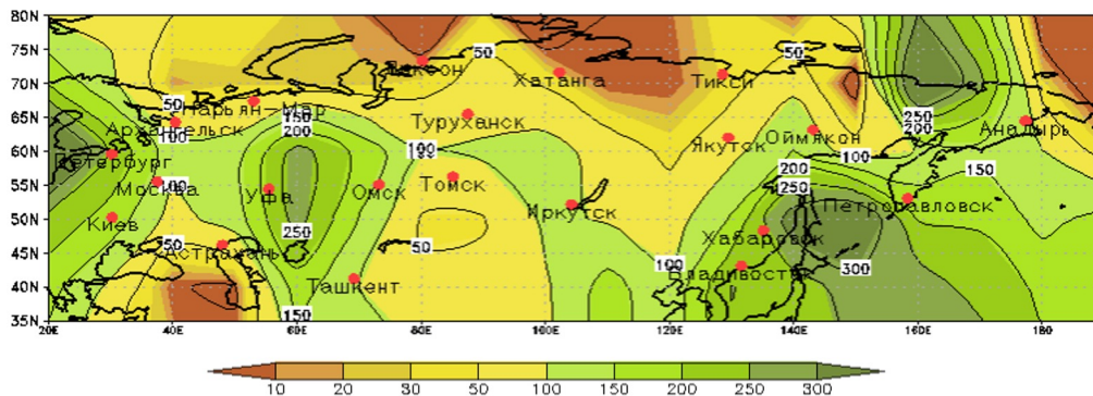
PRECIPITATION ANOMALIES (% from normal) 02.08-08.08.24 Observations (236 stations)
