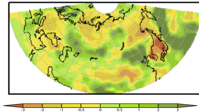
THE FORECAST OF PRECIPITATION ANOMALIES 09.08-15.08.24 Models SL-AV and MGO
