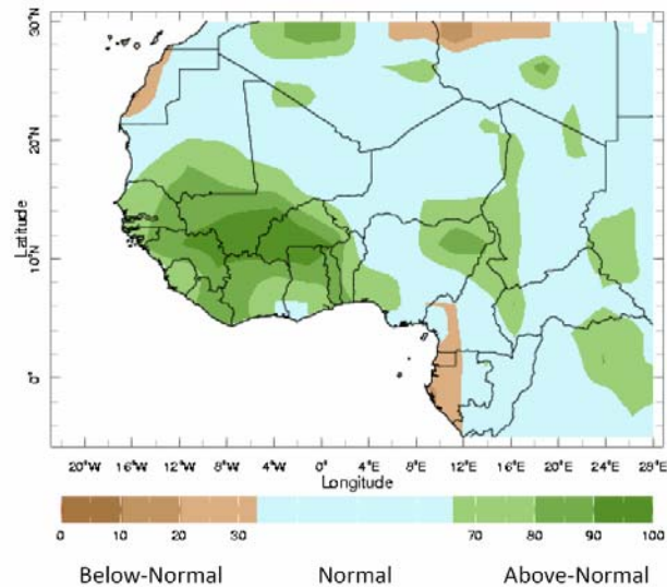
Figure 6. Example rainfall anomaly map for July – August 2008 with units in percentiles using a 1971 – 2000 climatology.
