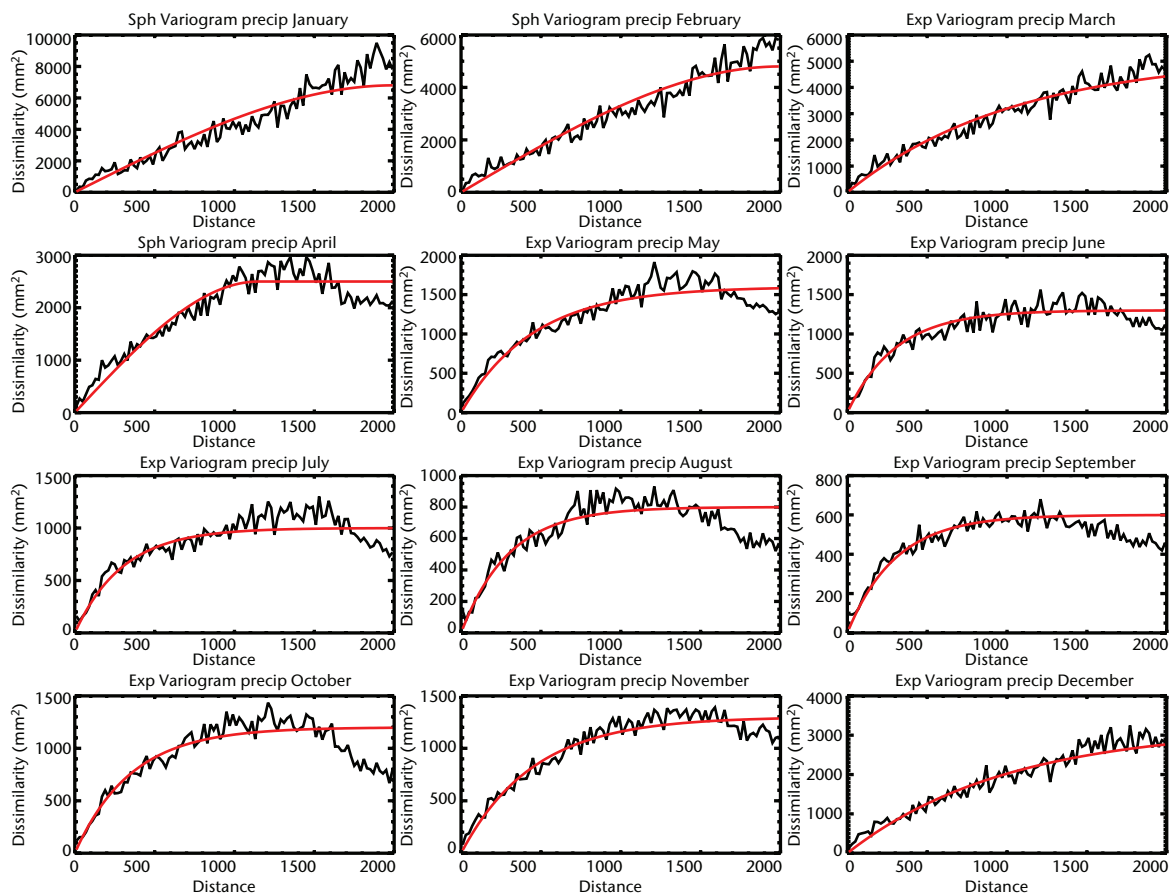
Figure 3. Sample variograms for Australian precipitation for each month from January (top left) to December (bottom right). The black lines are the empirical variograms. The red lines are the functional variograms. The average differences are typically small for small separations and increase as the separation of the stations increases.
