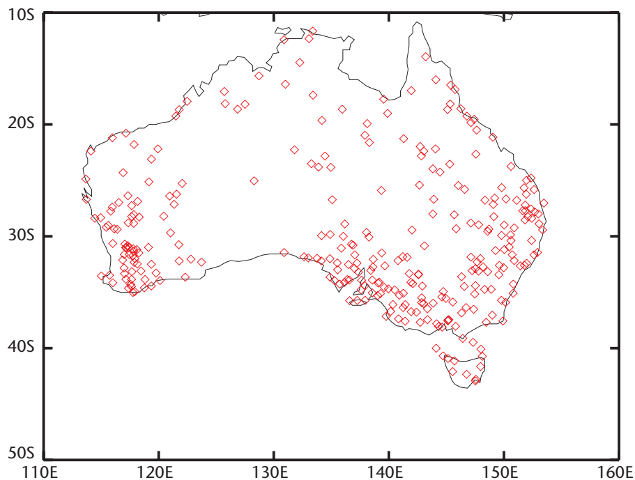
Figure 1. Station locations used to illustrate NCMP calculation (red diamonds) in Australia
