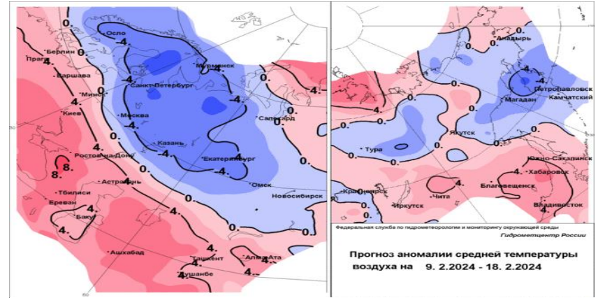
Forecast of T2m [K] anomalies. Models: HMC + MGO Forecast period: 09.02-15.02.2024, week 1
